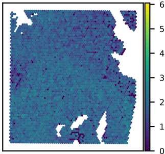
SNU51A HNRNPR expression Moran's I = 0.21
