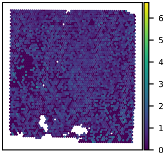
SNU43A GALNT11 expression Moran's I = 0.02
