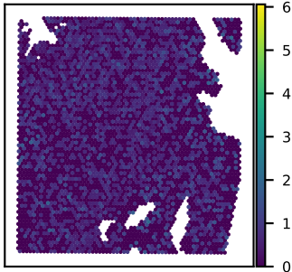
SNU51A PNPO expression Moran's I = 0.03
