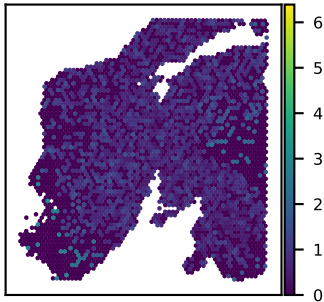
SNU24A TNFSF13B expression Moran's I = 0.05
