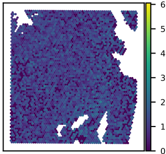
SNU51A ARMCX3 expression Moran's I = 0.03
