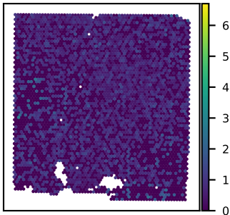
SNU43A SLC25A32 expression Moran's I = 0.02
