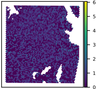
SNU51A MCCC1 expression Moran's I = 0.03
