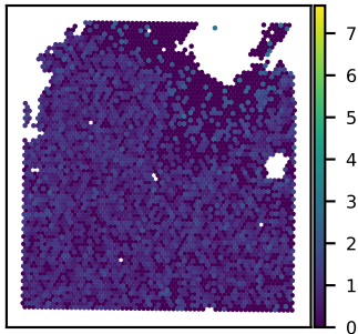
SNU21B GTF3C3 expression Moran's I = 0.05
