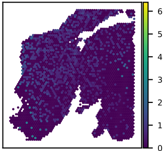
SNU24A CTNNA3 expression Moran's I = 0.09
