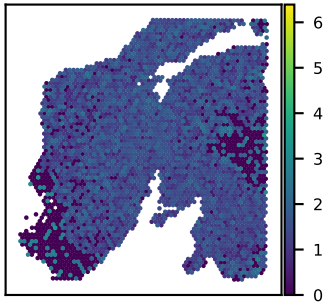
SNU24A NCSTN expression Moran's I = 0.15
