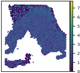
SNU18A CTDSP2 expression Moran's I = 0.16
