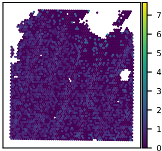
SNU21B ATPCKMT expression Moran's I = 0.03
