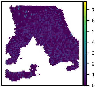
SNU18A CDCA7L expression Moran's I = 0.04
