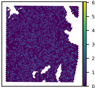
SNU51A GTF3C4 expression Moran's I = 0.01
