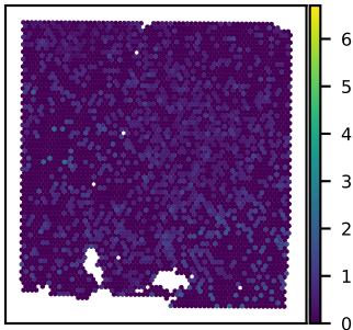
SNU43A VAMP1 expression Moran's I = 0.02
