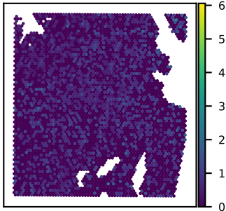
SNU51A WDR48 expression Moran's I = 0.03
