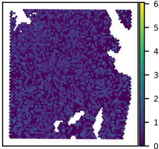
SNU51A TSEN15 expression Moran's I = 0.03
