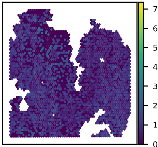
SNU27B CDKN1B expression Moran's I = 0.06
