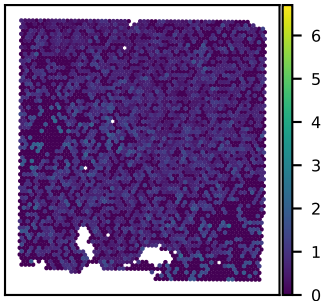
SNU43A TIMM9 expression Moran's I = 0.02
