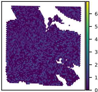
SNU24B SARM1 expression Moran's I = 0.01
