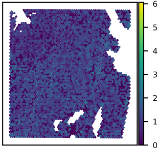
SNU51A PCNX2 expression Moran's I = 0.05
