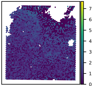
SNU21B SEPTIN11 expression Moran's I = 0.13
