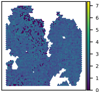
SNU27B LAMTOR4 expression Moran's I = 0.06
