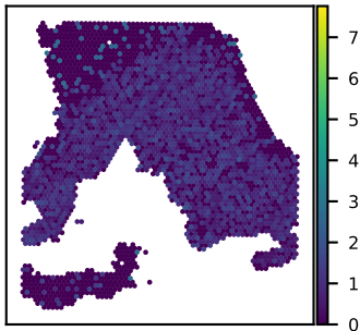
SNU18A PYCARD expression Moran's I = 0.15
