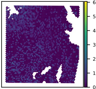
SNU51A CTHRC1 expression Moran's I = 0.09
