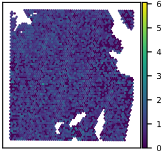
SNU51A ATRAID expression Moran's I = 0.03
