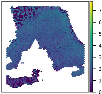
SNU18A PLXND1 expression Moran's I = 0.35
