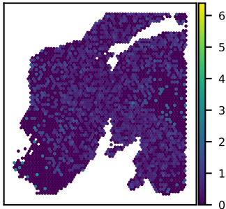
SNU24A CNST expression Moran's I = 0.03
