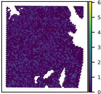
SNU51A RNF26 expression Moran's I = 0.02
