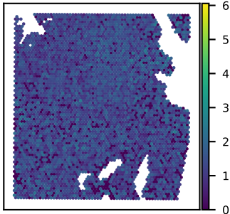
SNU51A CDS2 expression Moran's I = 0.03
