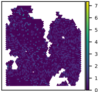
SNU27B CSNK2A3 expression Moran's I = 0.03
