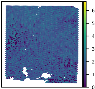
SNU43A KCTD12 expression Moran's I = 0.09
