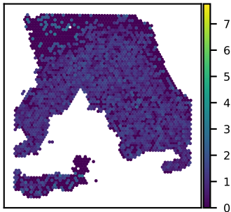
SNU18A EIF3H expression Moran's I = 0.13
