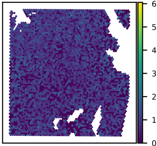
SNU51A POLDIP3 expression Moran's I = 0.02
