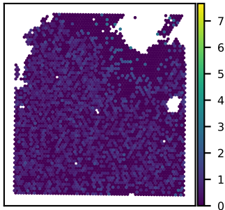
SNU21B CSNK1G3 expression Moran's I = 0.02
