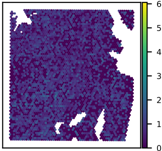
SNU51A TMEM8A expression Moran's I = 0.07
