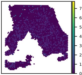
SNU18A C7orf25 expression Moran's I = 0.05
