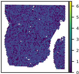
SNU25B SSBP1 expression Moran's I = 0.01
