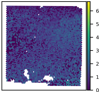
SNU43A ALDOC expression Moran's I = 0.19
