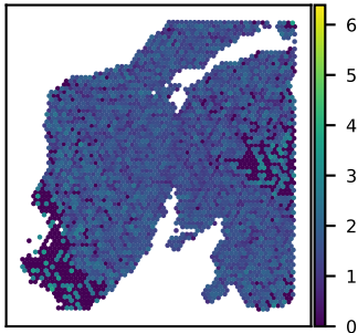
SNU24A MRFAP1L1 expression Moran's I = 0.10
