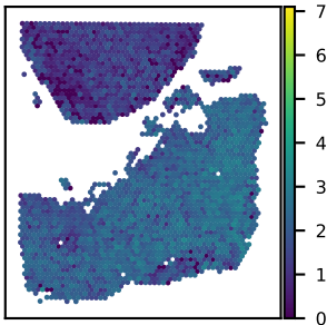
SNU25A TMEM144 expression Moran's I = 0.59
