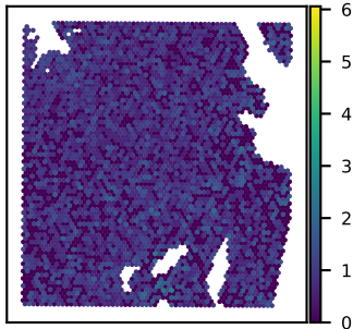
SNU51A SEC23A expression Moran's I = 0.03
