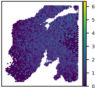
SNU24A SIGLEC1 expression Moran's I = 0.19
