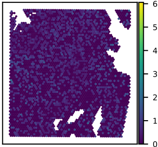
SNU51A SAP30L expression Moran's I = 0.01
