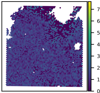
SNU21B PRELID3B expression Moran's I = 0.09
