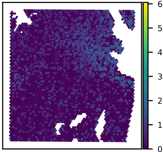
SNU51A PTK2B expression Moran's I = 0.25
