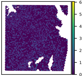
SNU51A PDLIM7 expression Moran's I = 0.02
