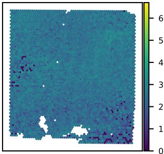
SNU43A CNN3 expression Moran's I = 0.23
