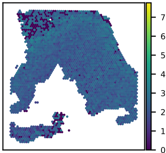
SNU18A CAPZA2 expression Moran's I = 0.20
