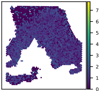
SNU18A PAPSS1 expression Moran's I = 0.13
